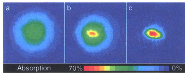
FIG. 2 (color). Two-dimensional probe absorption images, after 6 ms time of flight, showing evidence for BEC. (a) is the velocity distribution of a cloud cooled to just above the transition point, (b) just after the condensate appeared, and (c) after further evaporative cooling has left an almost pure condensate. (b) shows the difference between the isotropic thermal distribution and an elliptical core attributed to the expansion of a dense condensate. The width of the images is 870 \mu\text{m} . Gravitational acceleration during the probe delay displaces the cloud by only 0.2 mm along the z axis.
