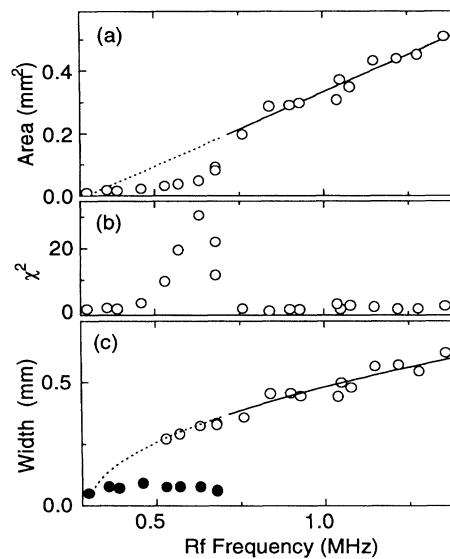
FIG. 4. Further evidence for a phase transition is provided by the sudden change of observed quantities as the final rf frequency \nu_{\text{rf}} is varied. (a) Area of the cloud in the time-of-flight image versus \nu_{\text{rf}} . The area was obtained as the ratio of the integrated optical density and the peak optical density. The area changes suddenly at \nu_{\text{rf}} = 0.7 MHz. Below the same frequency, the velocity distributions (Fig. 3) cannot be represented by a single Gaussian, as demonstrated by the \chi^2 for a single Gaussian fit (b), and required different widths for the condensate (full circles) and noncondensate fraction (c). In (a) and (c) the lines reflect the behavior of a classical gas with a temperature proportional to the trap depth.
